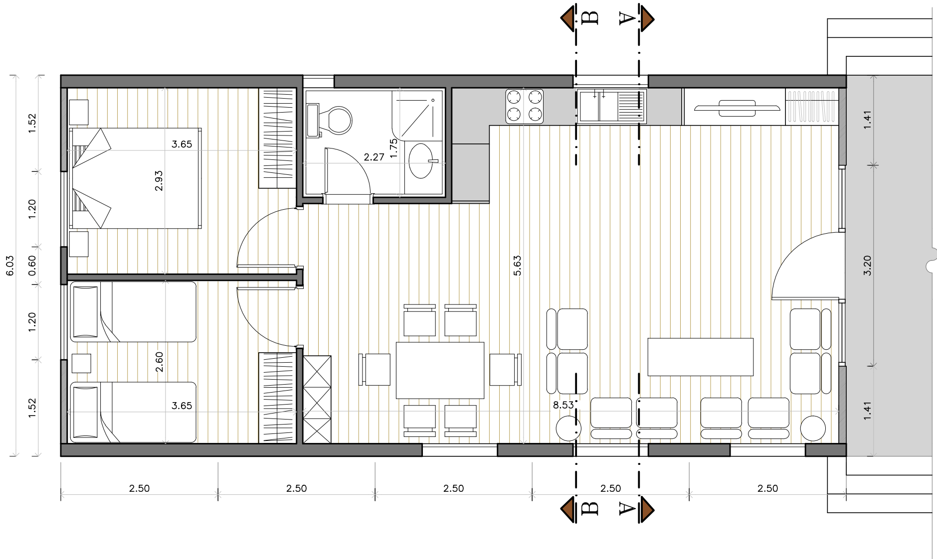
Ground Floor Plan (5 modules)
