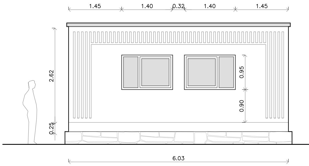
Back Elevation
